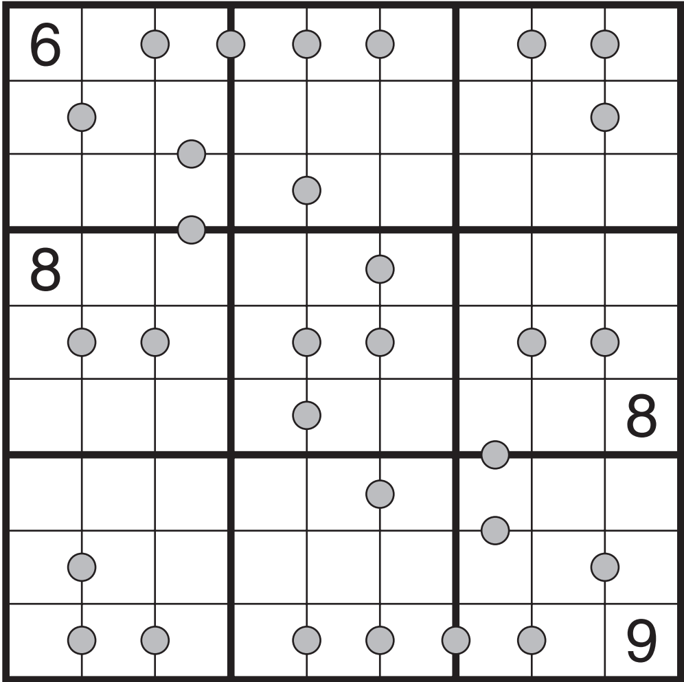
Complete Symmetry
